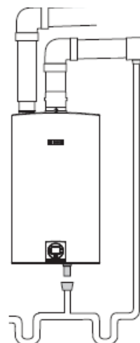
Sample Twin Pipe Venting Installation
